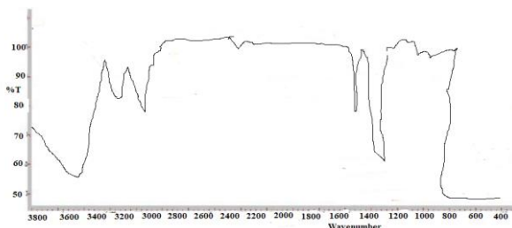
Fig. FTIR Spectra of Dowex -50
