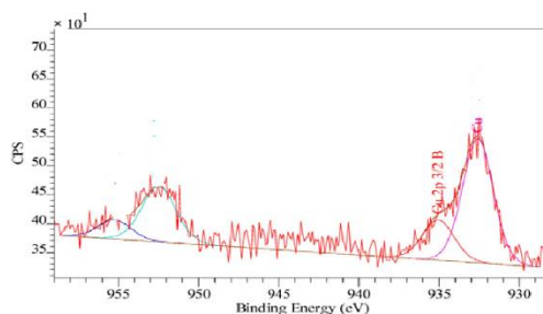
XPS spectrum obtained in a wide range of binding energy made for the Dowex 50 With Pregabalin sorption
