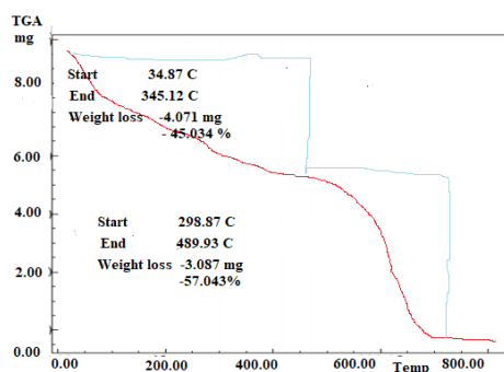
Fig. TGA for 30% condensate resin
