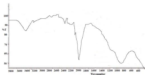
Fig. FTIR Spectra of Pregabalin
