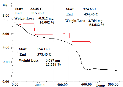
Fig. TGA for pure drug
